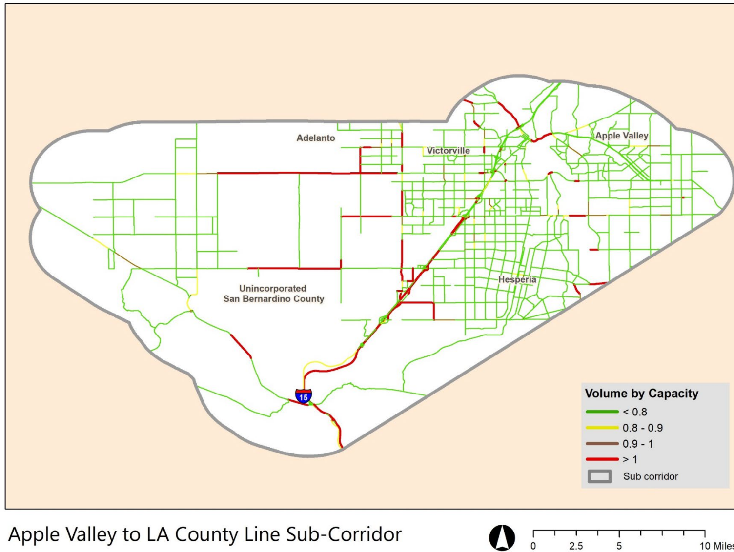
Figure 5.54 | Future 2040 Traffic Conditions—PM Apple Valley to Los Angeles County Line Sub-Corridor
